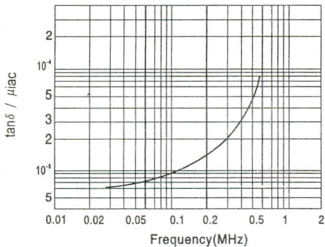
\tan\delta / \mu_{iac} Vs. frequency response characteristics (L-series materials)
