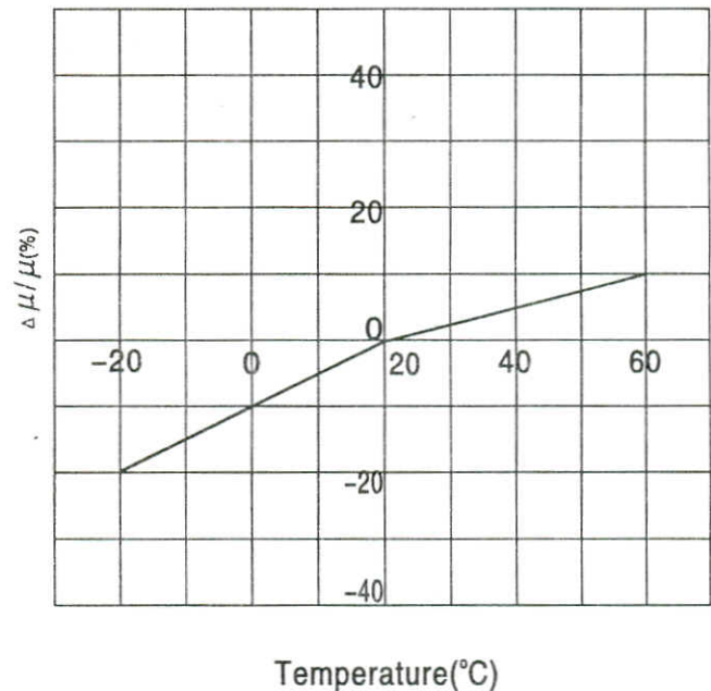
\Delta \mu / \mu Vs. temperature curve (L-series materials)
