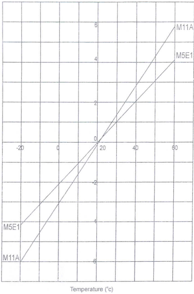
\Delta \mu / \mu Vs. temperature curve (M-series materials)
