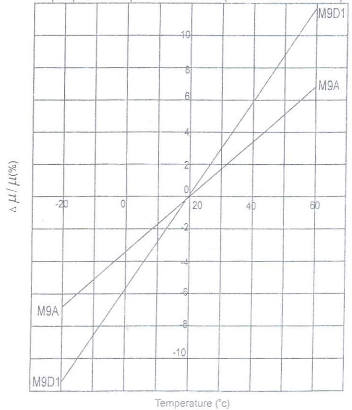
\Delta \mu / \mu Vs. temperature curve (M-series materials)
