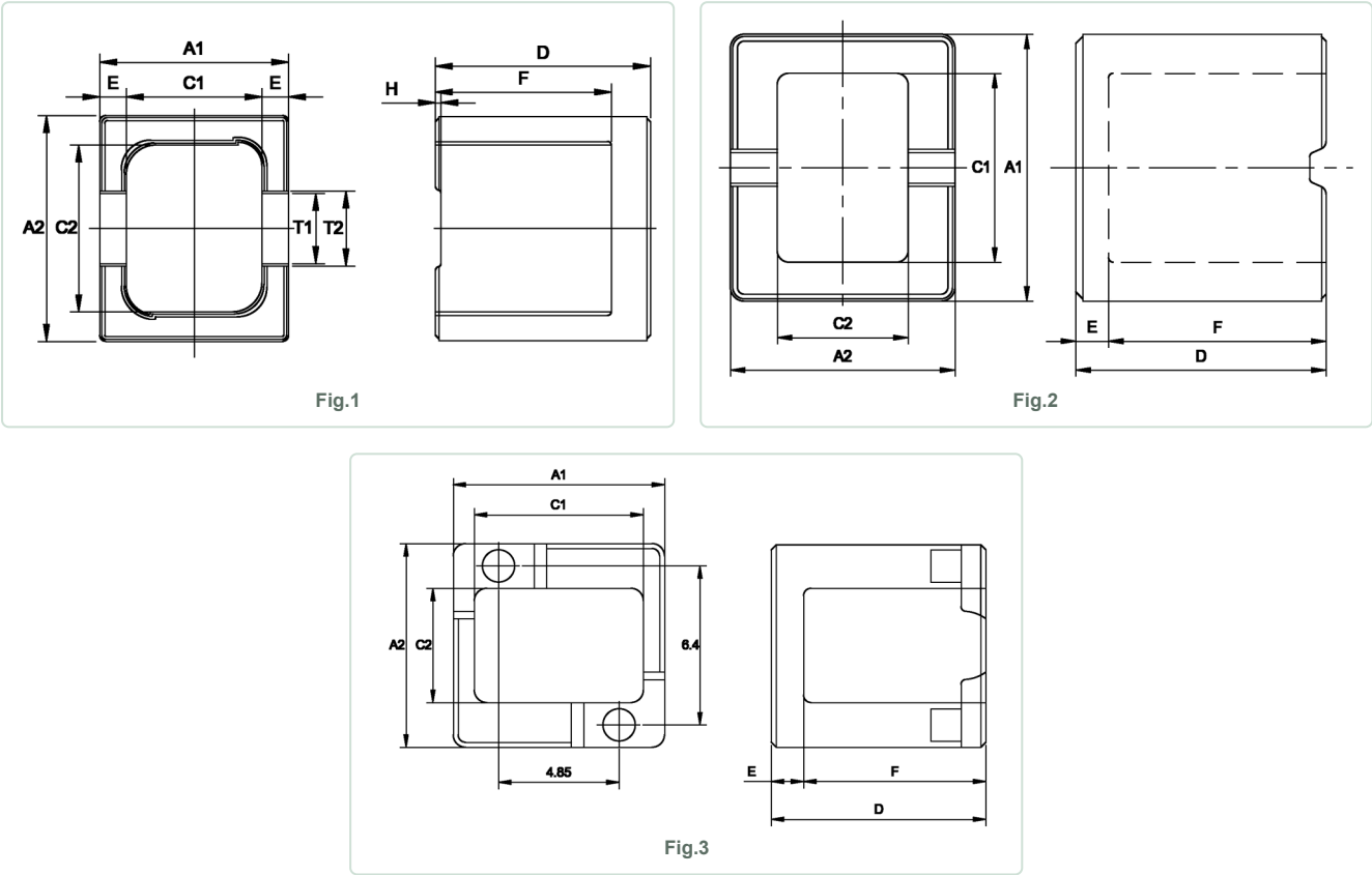
SP POT CORES (CPU CHOKE) — OUTLINE DRAWINGS (FIG.1-3)
