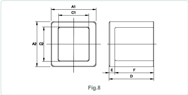
SP POT CORES (CPU CHOKE) — OUTLINE DRAWINGS ( FIG.7-9 )
